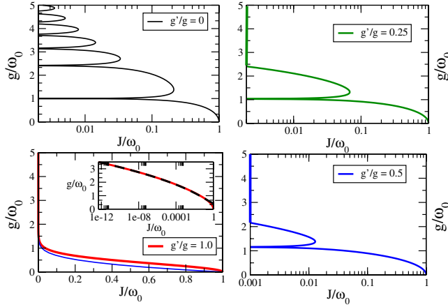
FIG. 3 (color online). Mean field phase diagram for the generalized Rabi lattice model for different values of g'/g . For the Rabi case g' = g , we compare with the mean field phase diagram for the effective spin model (bottom left panel). In the inset, we show the decay of the critical coupling J_c at ultrastrong coupling J_c = \omega_0^3 e^{-2(g/\omega_0)^2} / 4g^2 [45]
