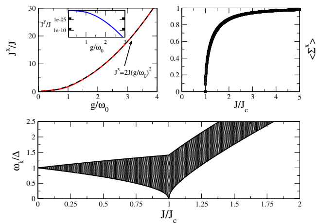
FIG. 2 (color online). Top left panel: scaled ferromagnetic coupling J^{x,y}/J of the effective spin model as a function of g/\omega_0 . While J^x \sim (g/\omega_0)^2 at ultrastrong coupling, the coupling along y is vanishingly small. Top right panel: mean-field order parameter for the effective spin model. Bottom panel: band of spin-wave excitations above the ground state.
