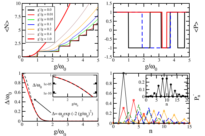
FIG. 1 (color online). Evolution of single-site generalized Rabi model ground state properties upon increasing the strength of counterrotating terms g'/g . Top panels: number of excitations and parity of the ground state as a function of g/\omega_0 and for different g'/g . Bottom panels: (left) decay of level splitting \Delta in the ultrastrong coupling regime and (right) probability of having n polaritons in the Rabi ground state (inset) and its evolution with g'/g = 0.0, 0.25, 0.5, 0.75 , and 1.0 .
